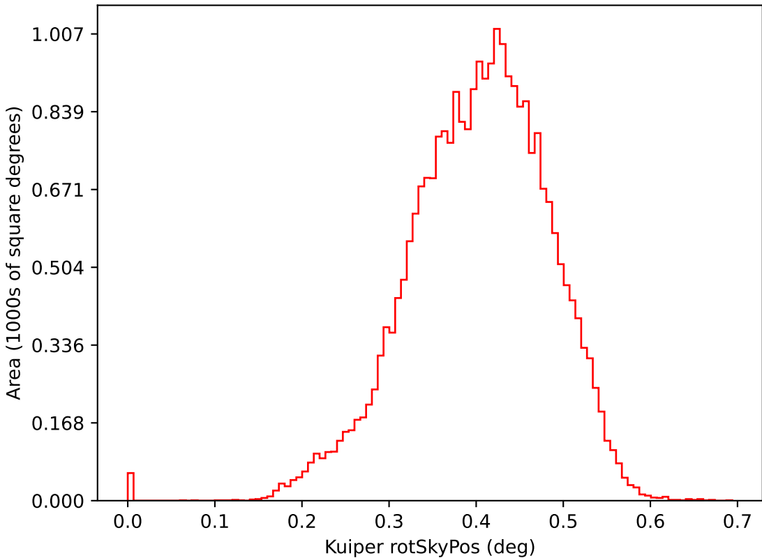
too_elab_r8_d3_giz_v3.4_10yrs i: Kuiper rotSkyPos
