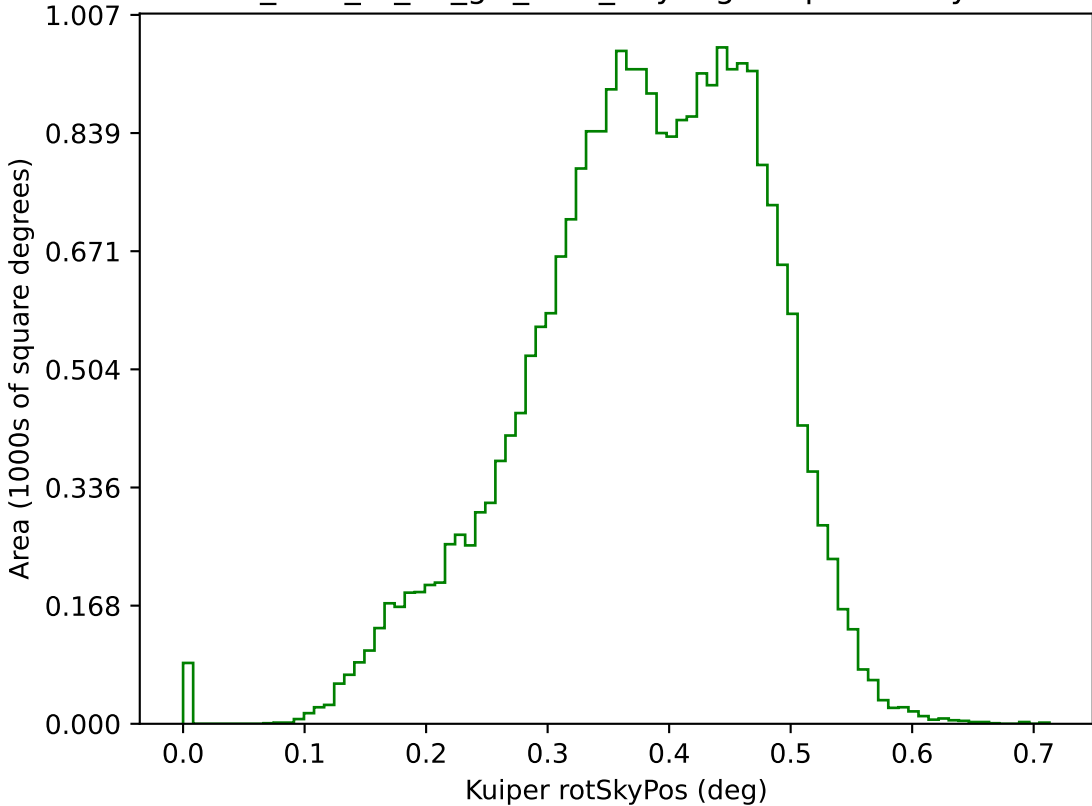
too_elab_r8_d3_giz_v3.4_10yrs g: Kuiper rotSkyPos
