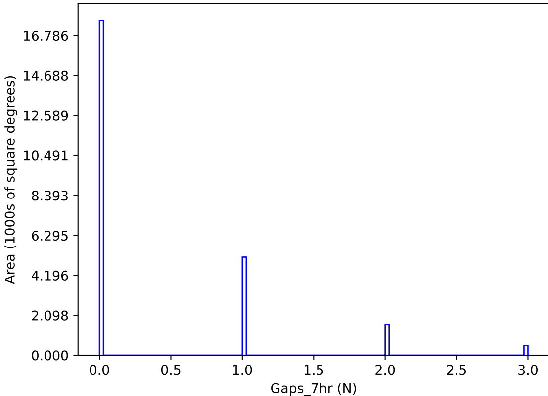
too_elab_r8_d3_giz_v3.4_10yrs y band: Gaps_7hr
