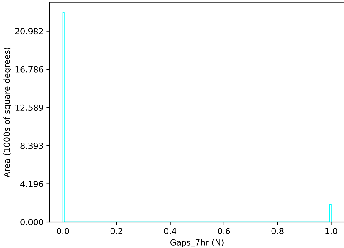
too_elab_r8_d3_giz_v3.4_10yrs u band: Gaps_7hr
