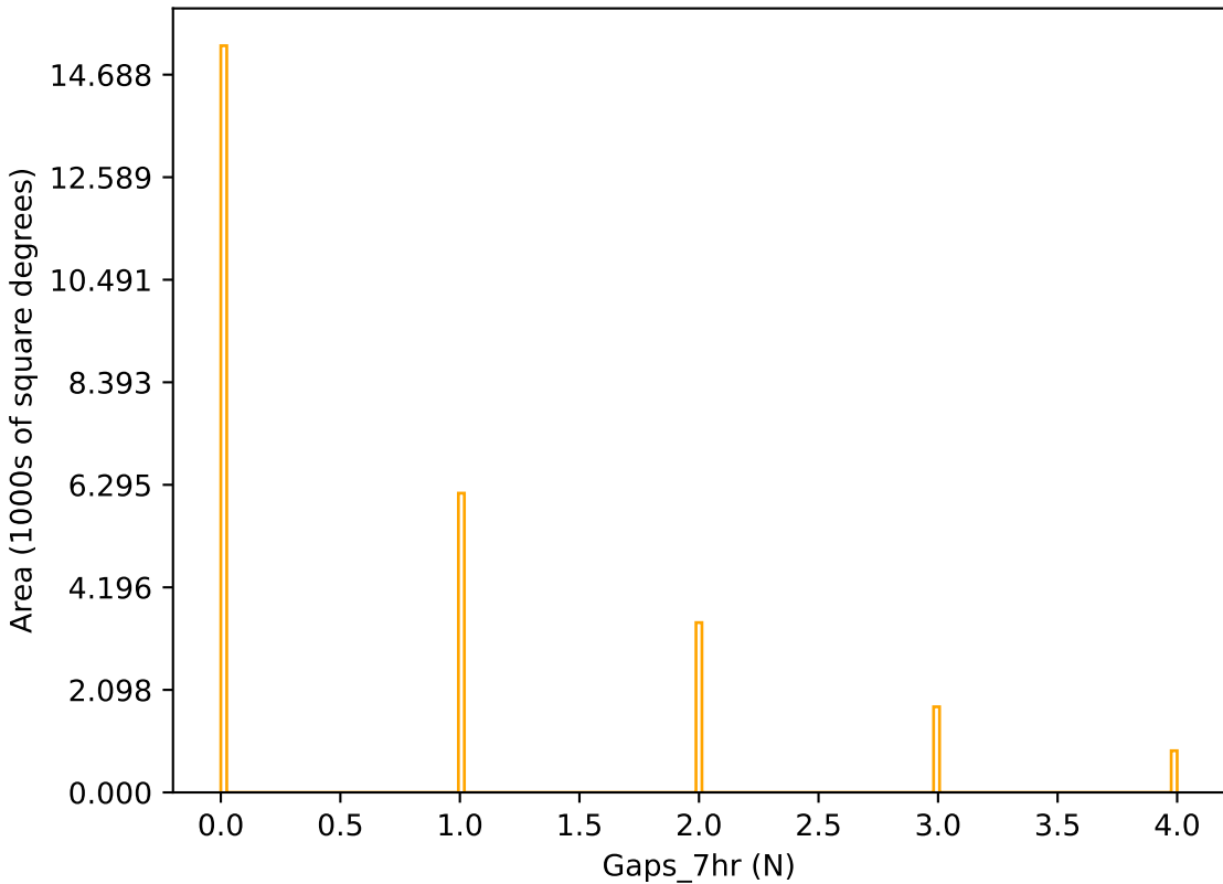
too_elab_r8_d3_giz_v3.4_10yrs r band: Gaps_7hr
