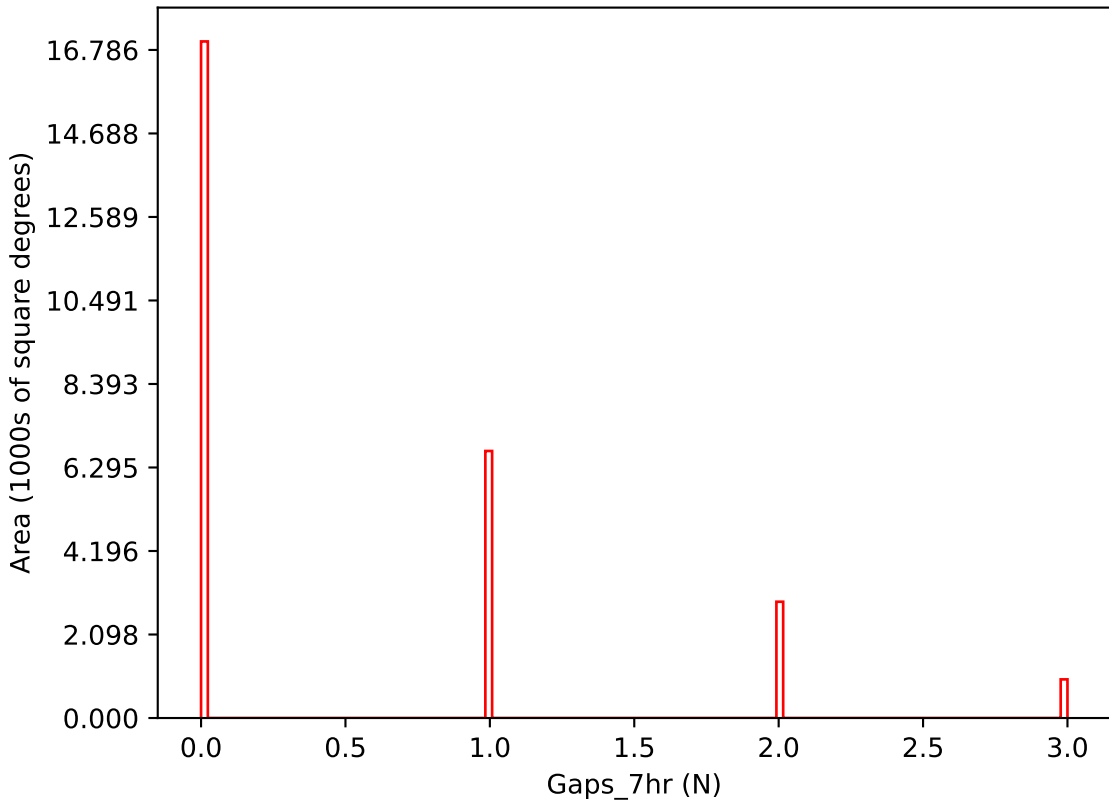
too_elab_r8_d3_giz_v3.4_10yrs i band: Gaps_7hr
