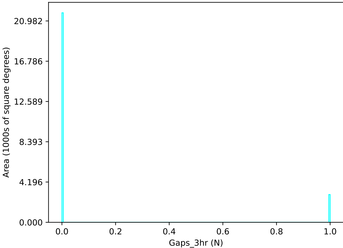
too_elab_r8_d3_giz_v3.4_10yrs u band: Gaps_3hr
