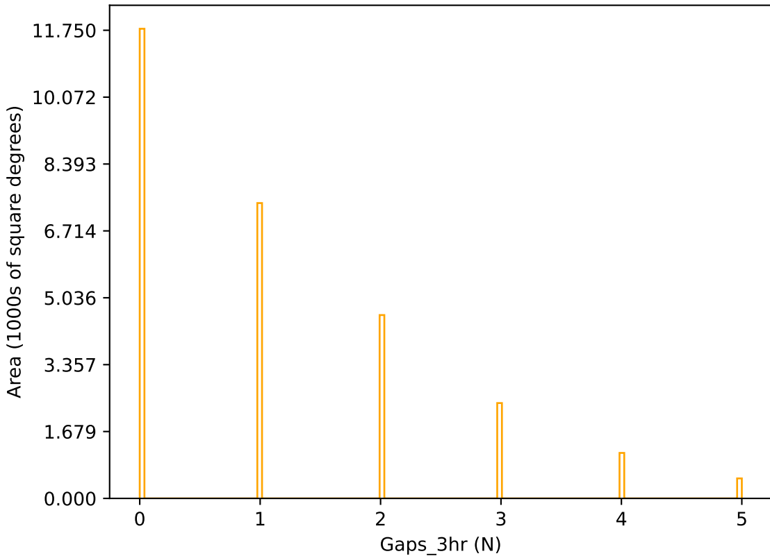
too_elab_r8_d3_giz_v3.4_10yrs r band: Gaps_3hr
