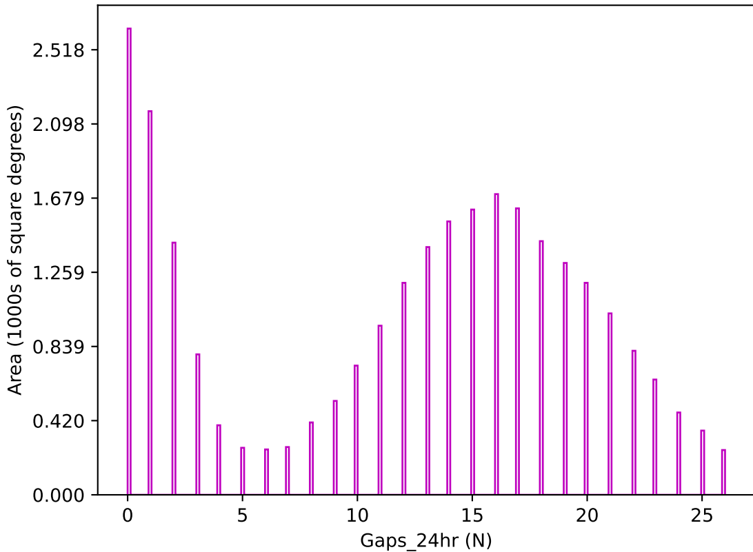
too_elab_r8_d3_giz_v3.4_10yrs z band: Gaps_24hr
