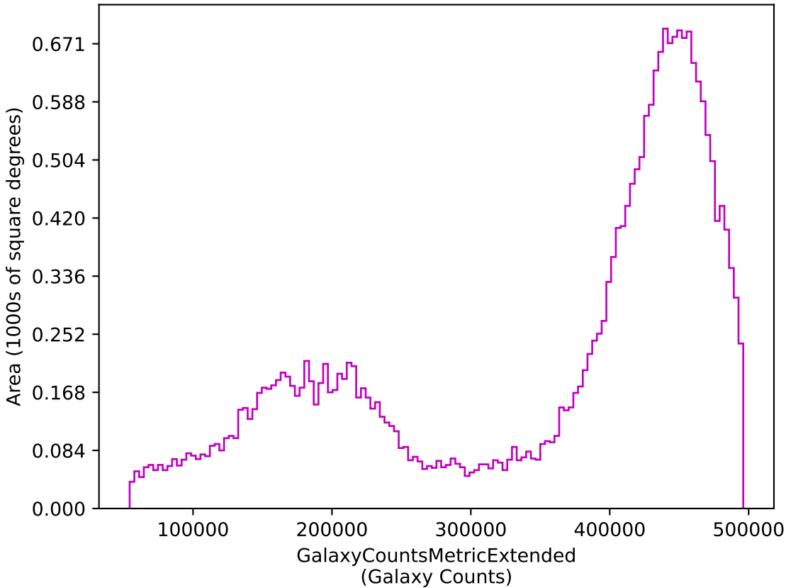
too_elab_r8_d3_giz_v3.4_10yrs z: GalaxyCountsMetricExtended
