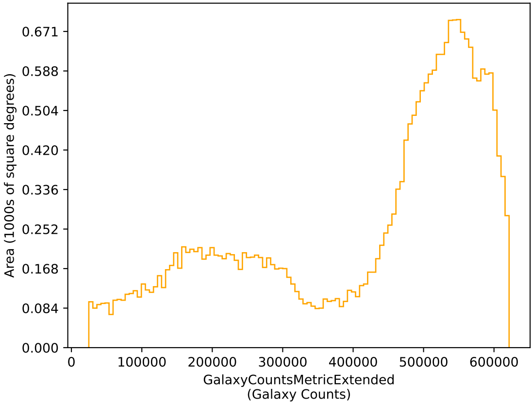
too_elab_r8_d3_giz_v3.4_10yrs r: GalaxyCountsMetricExtended
