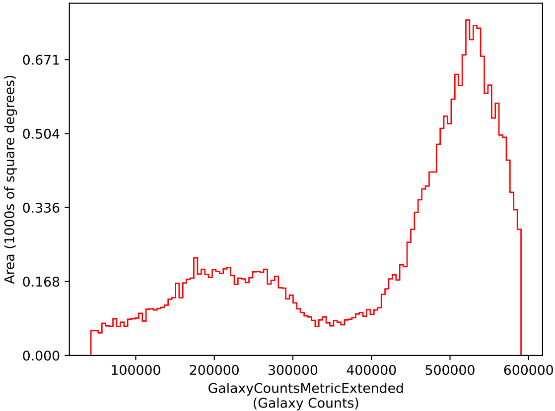
too_elab_r8_d3_giz_v3.4_10yrs i: GalaxyCountsMetricExtended
