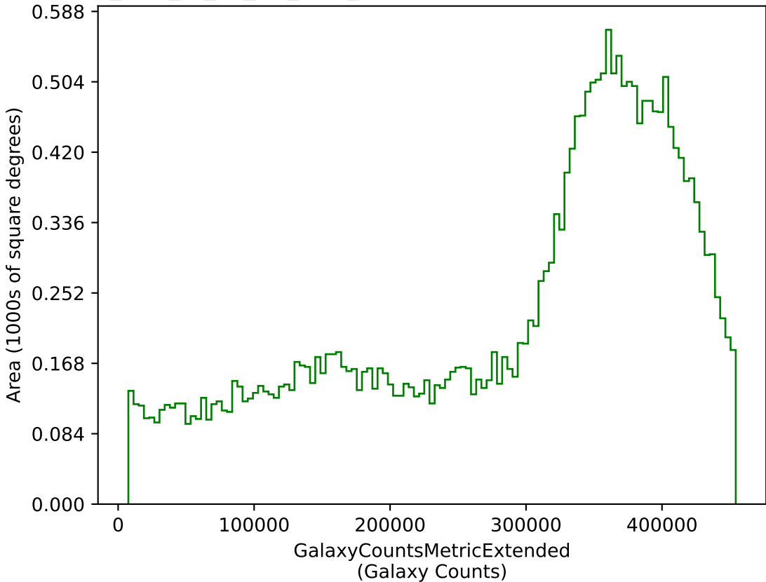
too_elab_r8_d3_giz_v3.4_10yrs g: GalaxyCountsMetricExtended
