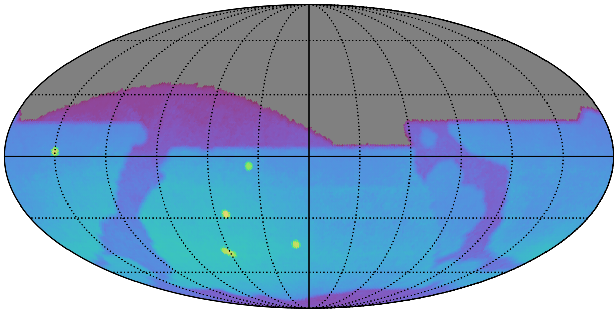
too_elab_r8_d3_giz_v3.4_10yrs : Brown Dwarf, L7
