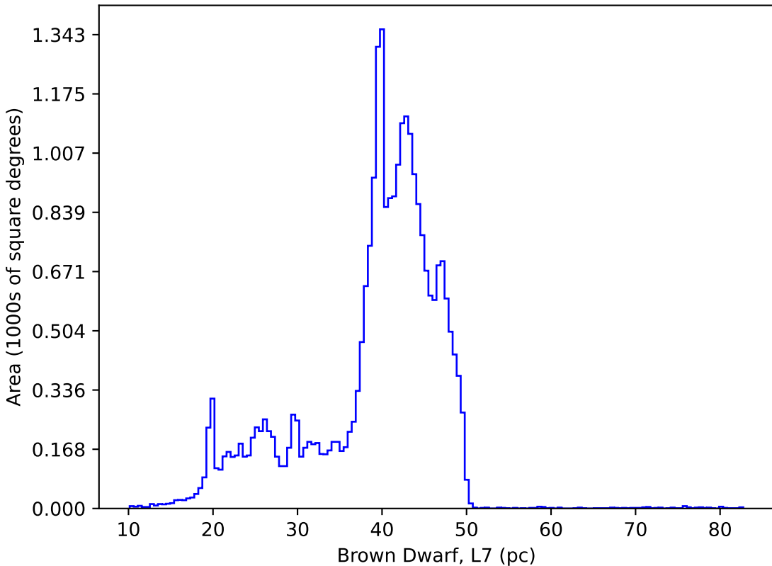
too_elab_r8_d3_giz_v3.4_10yrs : Brown Dwarf, L7
