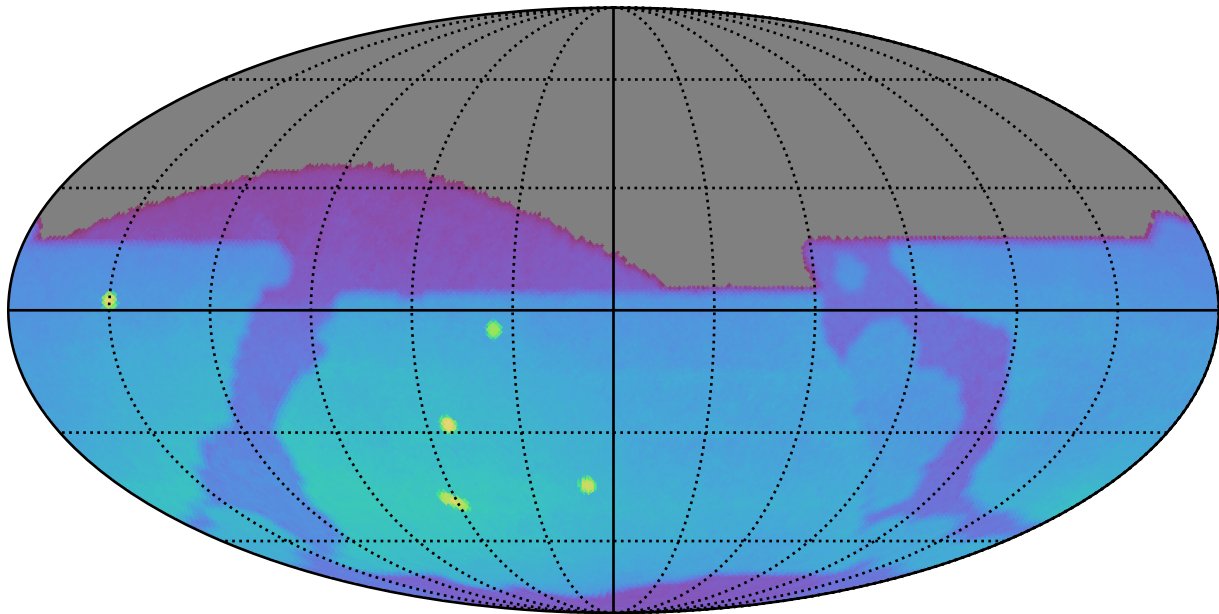
too_elab_r8_d3_giz_v3.4_10yrs : Brown Dwarf, L4
