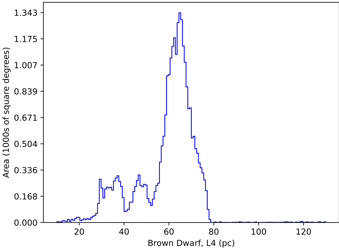
too_elab_r8_d3_giz_v3.4_10yrs : Brown Dwarf, L4
