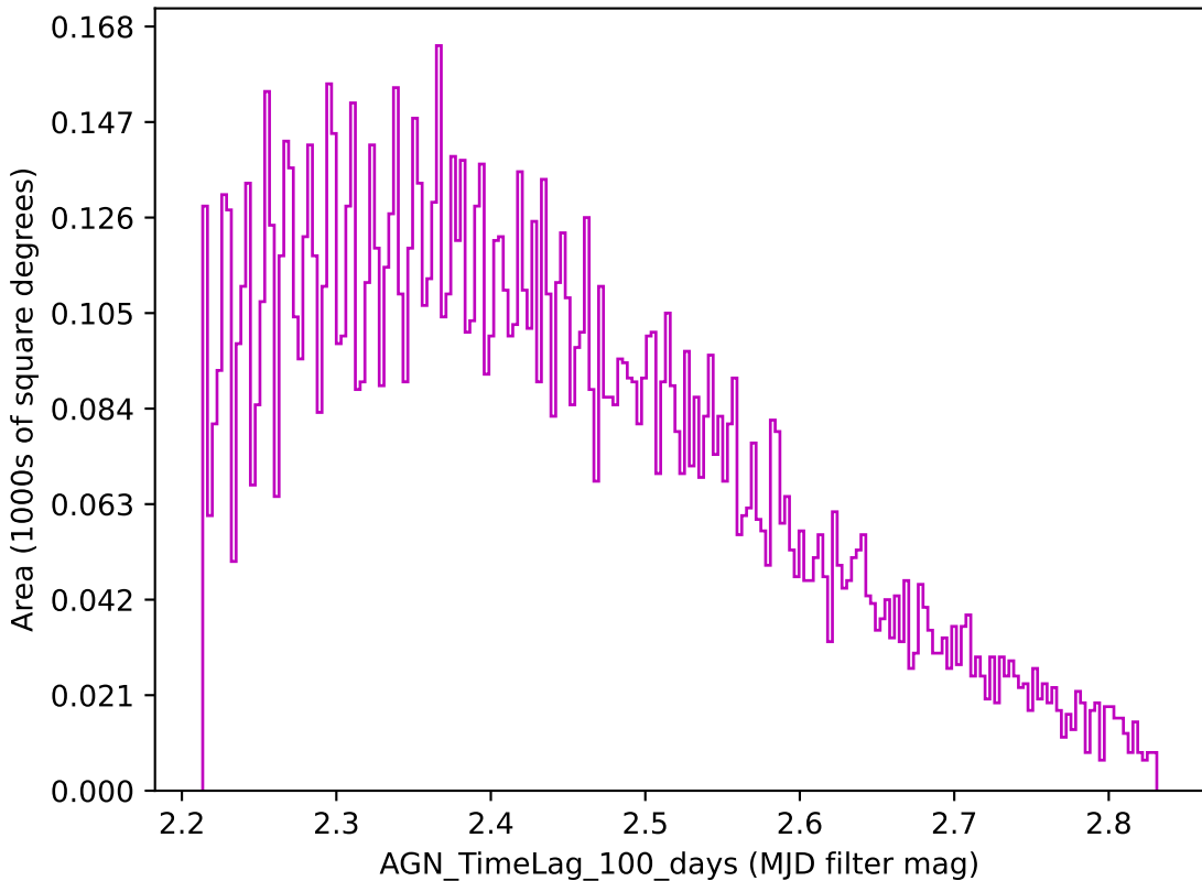
too_elab_r8_d3_giz_v3.4_10yrs z band: AGN_TimeLag_100_days
