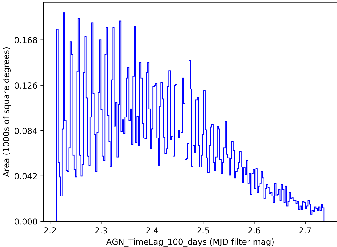
too_elab_r8_d3_giz_v3.4_10yrs y band: AGN_TimeLag_100_days
