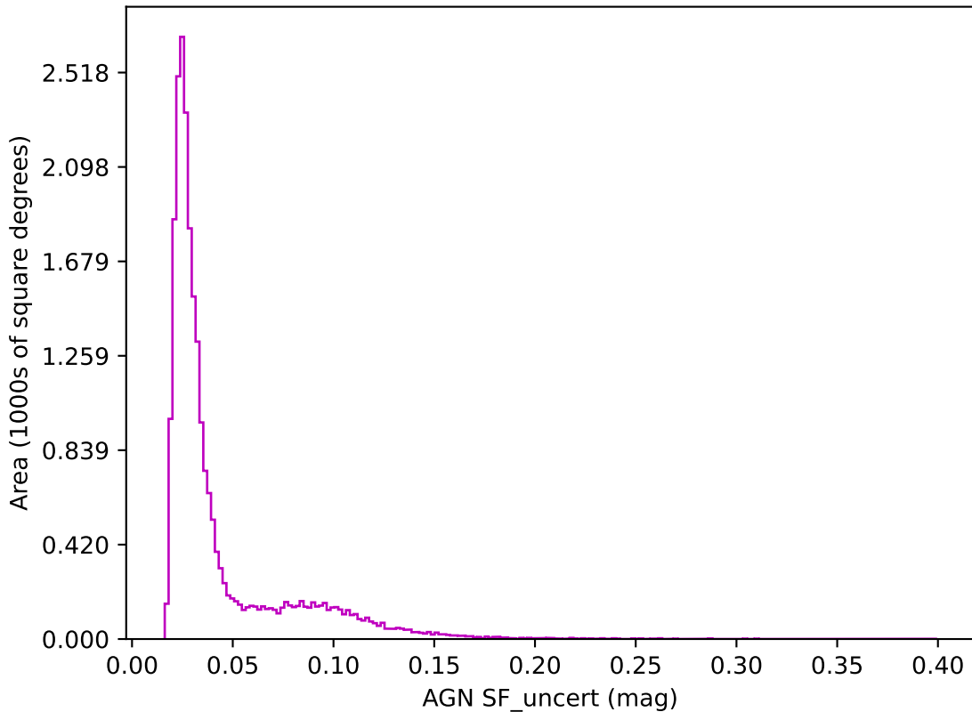
too_elab_r8_d3_giz_v3.4_10yrs z band: AGN SF_uncert
