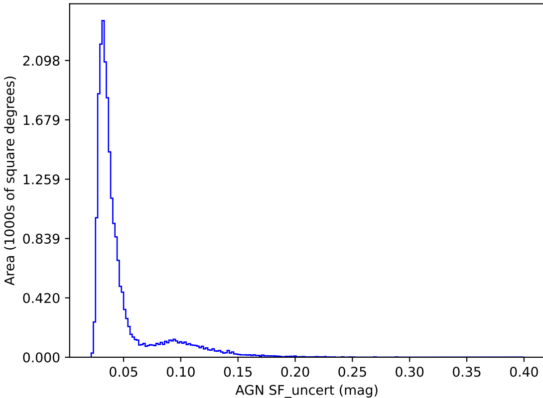
too_elab_r8_d3_giz_v3.4_10yrs y band: AGN SF_uncert
