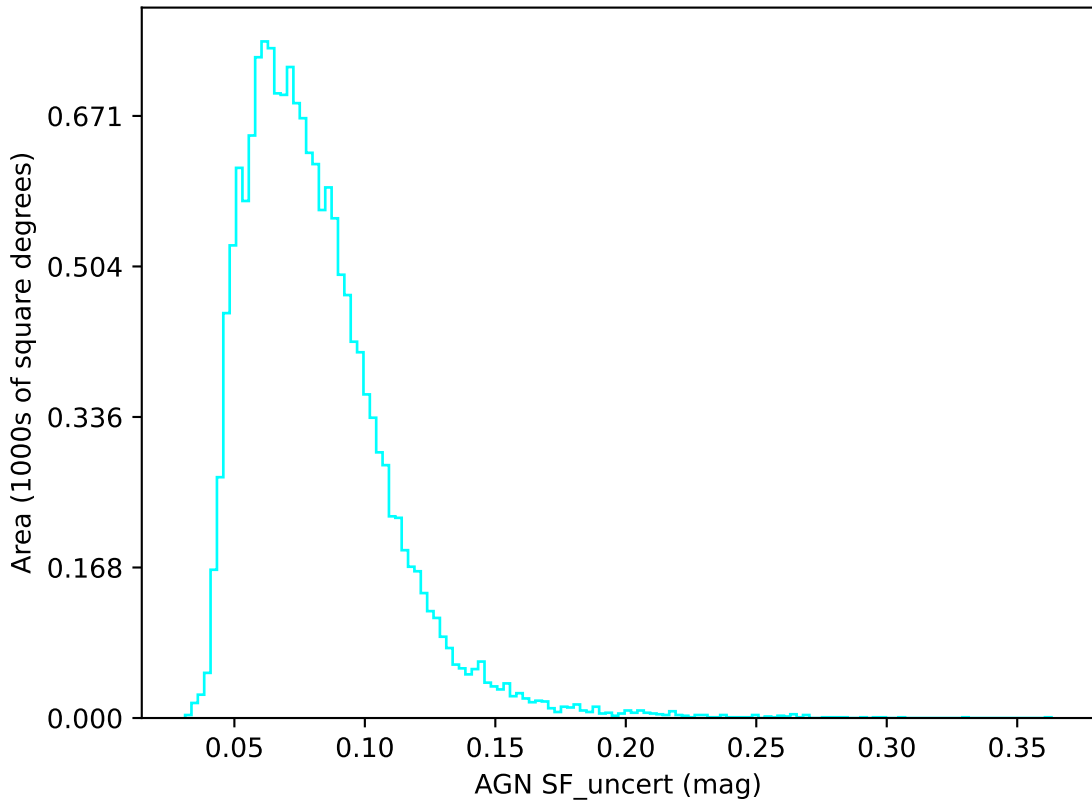
too_elab_r8_d3_giz_v3.4_10yrs u band: AGN SF_uncert
