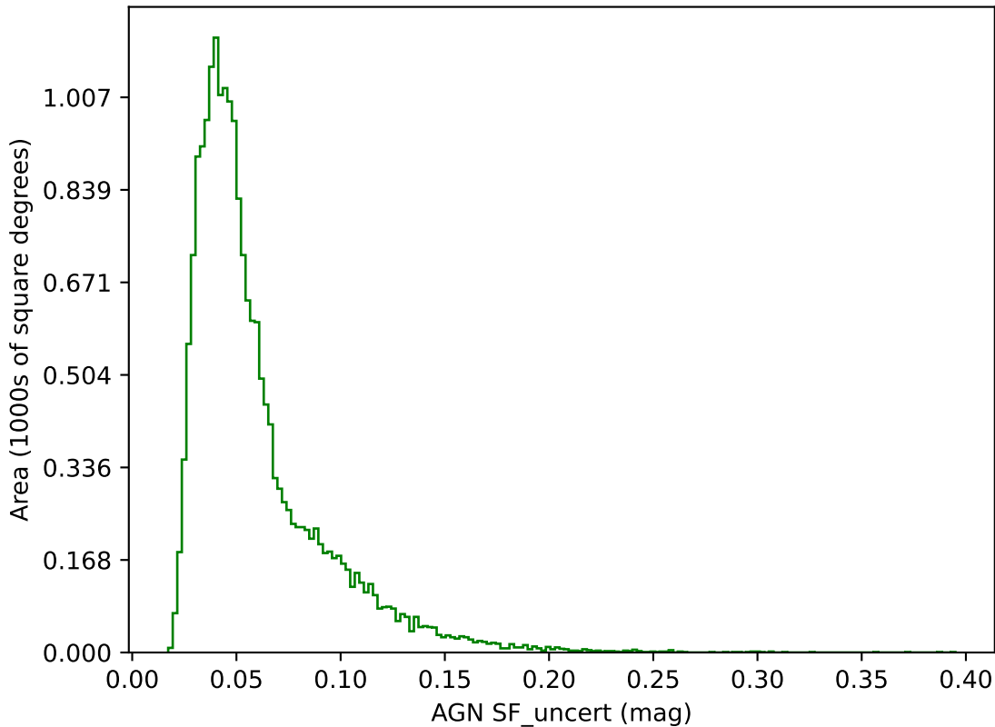
too_elab_r8_d3_giz_v3.4_10yrs g band: AGN SF_uncert
