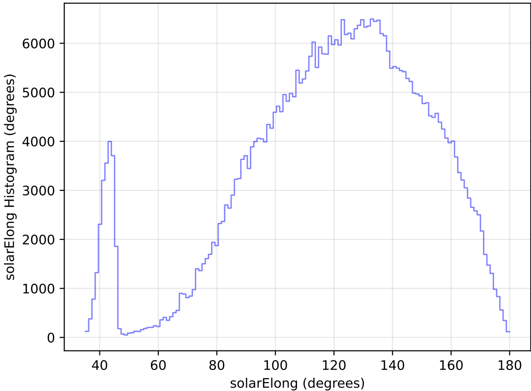
too_elab_r8_d3_giz_v3.4_10yrs WFD z band: solarElong Histogram
