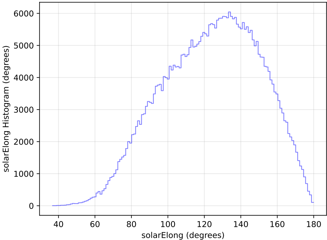
too_elab_r8_d3_giz_v3.4_10yrs WFD y band: solarElong Histogram
