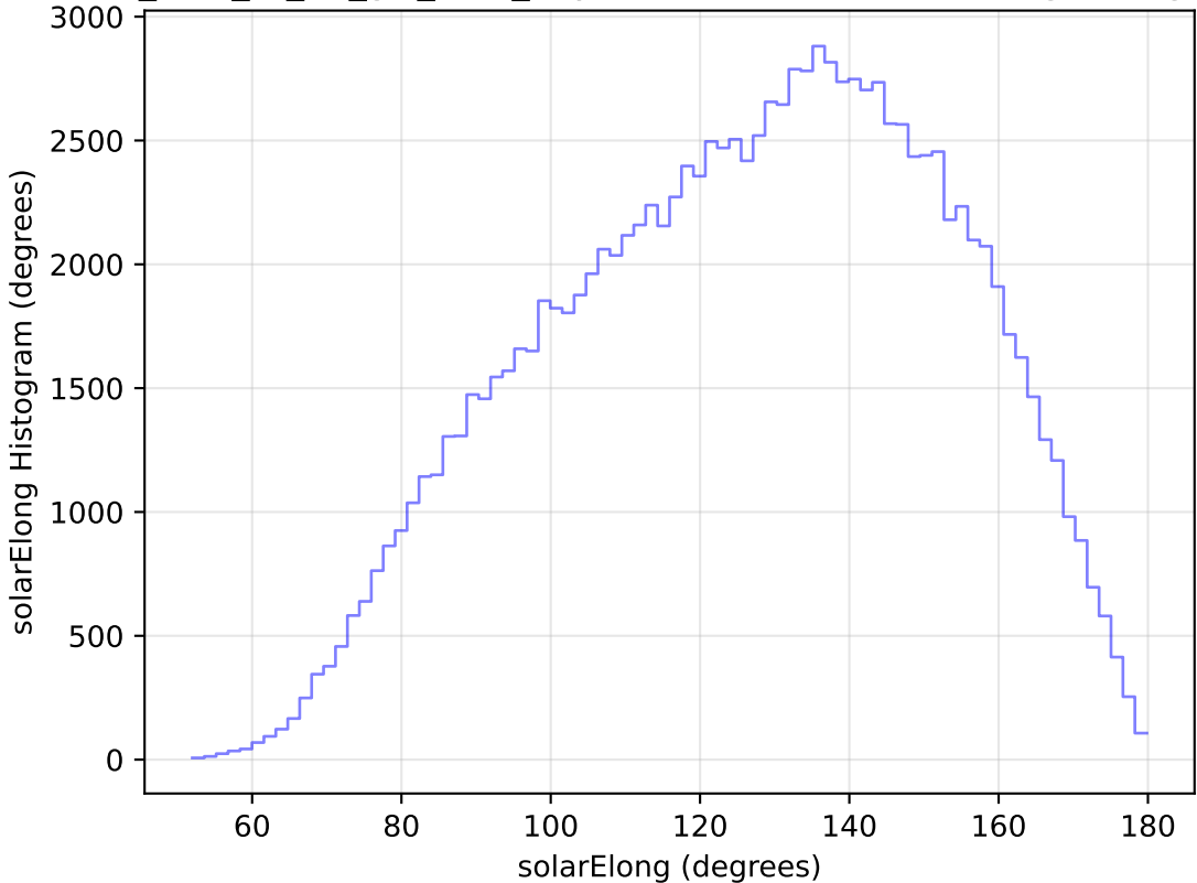
too_elab_r8_d3_giz_v3.4_10yrs WFD u band: solarElong Histogram
