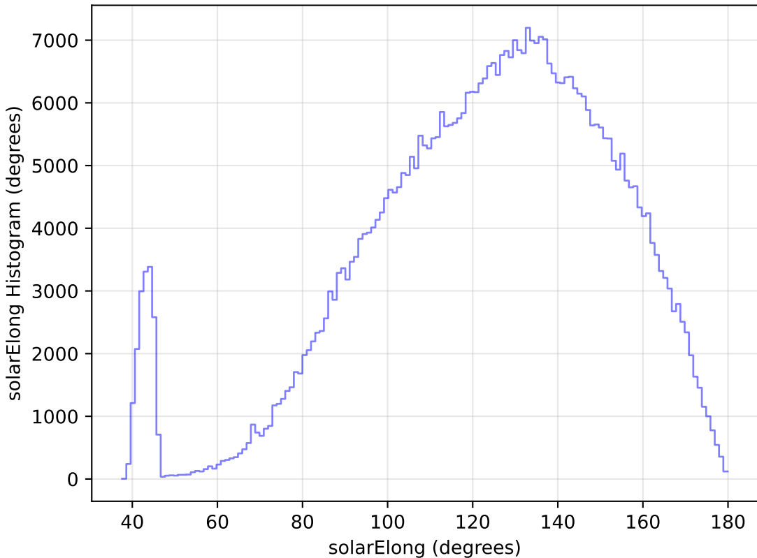
too_elab_r8_d3_giz_v3.4_10yrs WFD r band: solarElong Histogram
