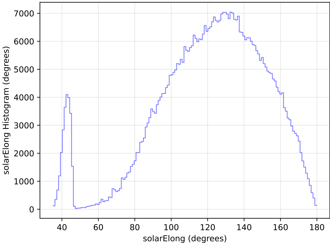
too_elab_r8_d3_giz_v3.4_10yrs WFD i band: solarElong Histogram
