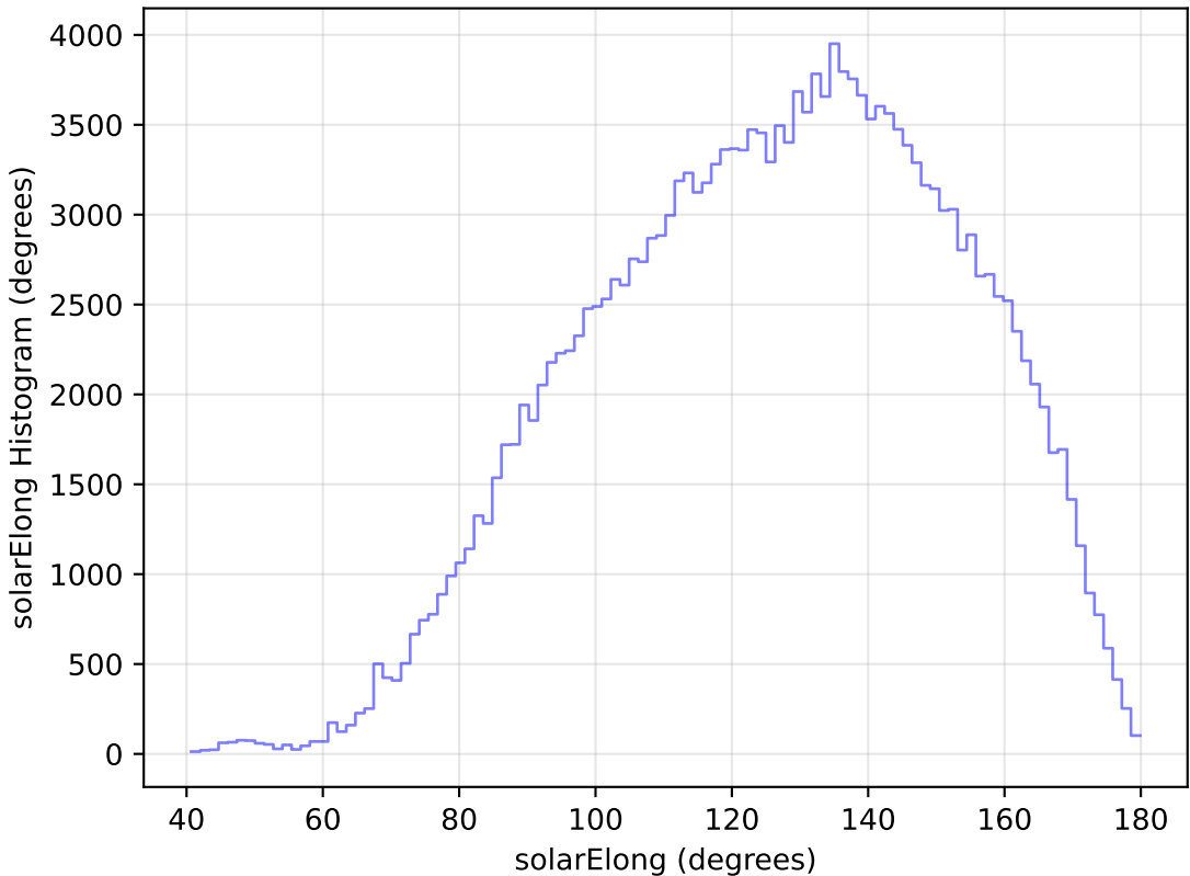
too_elab_r8_d3_giz_v3.4_10yrs WFD g band: solarElong Histogram
