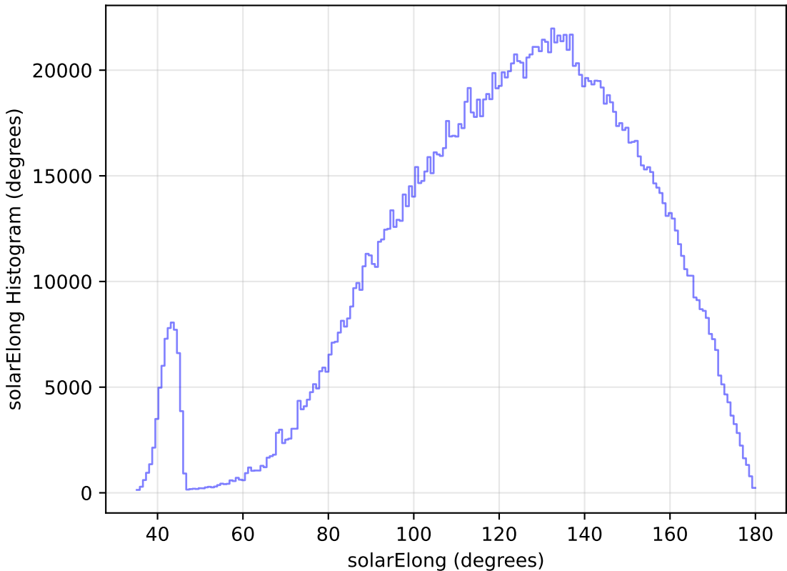
too_elab_r8_d3_giz_v3.4_10yrs WFD all bands: solarElong Histogram
