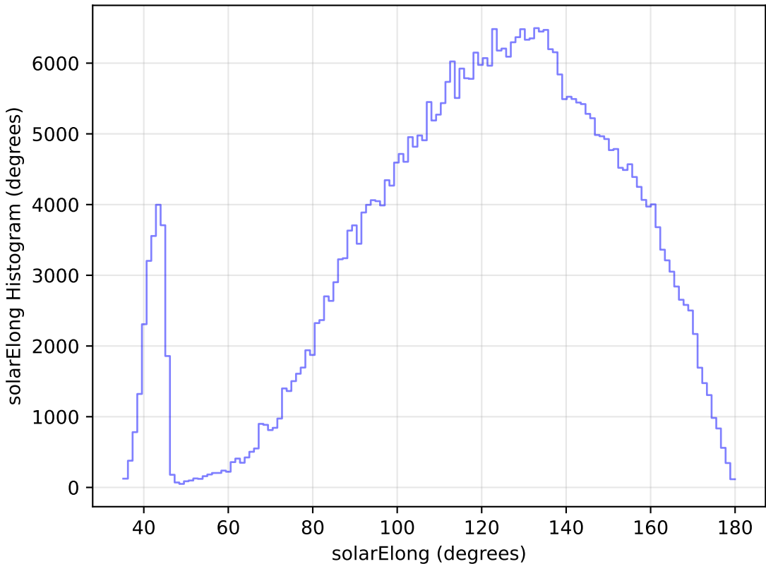
too_elab_r8_d3_giz_v3.4_10yrs All sky z band: solarElong Histogram
