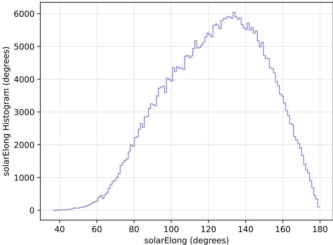
too_elab_r8_d3_giz_v3.4_10yrs All sky y band: solarElong Histogram
