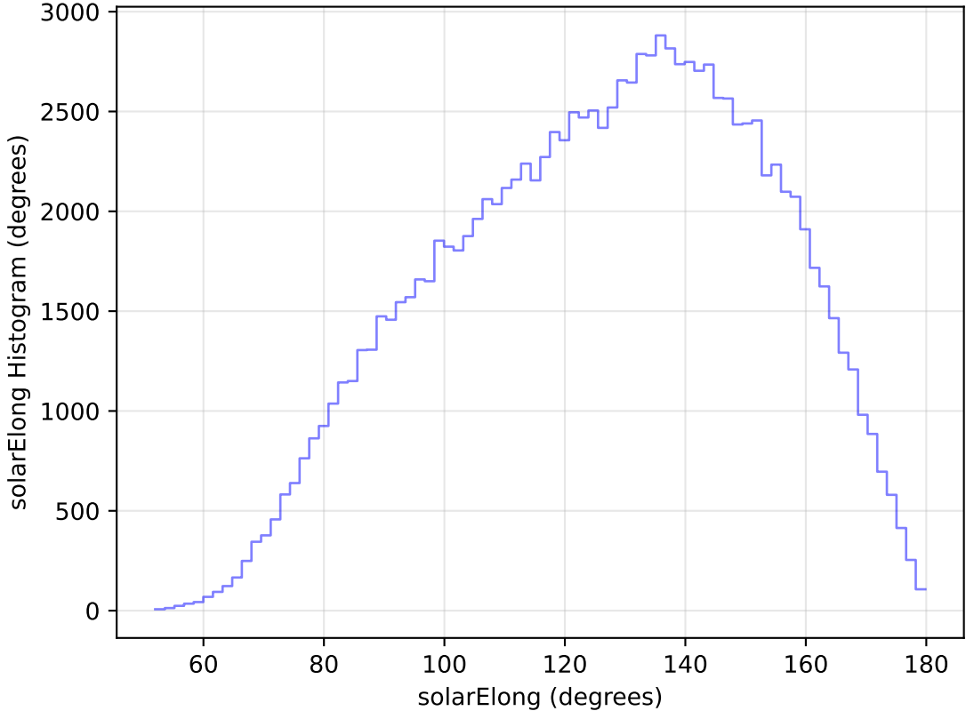
too_elab_r8_d3_giz_v3.4_10yrs All sky u band: solarElong Histogram
