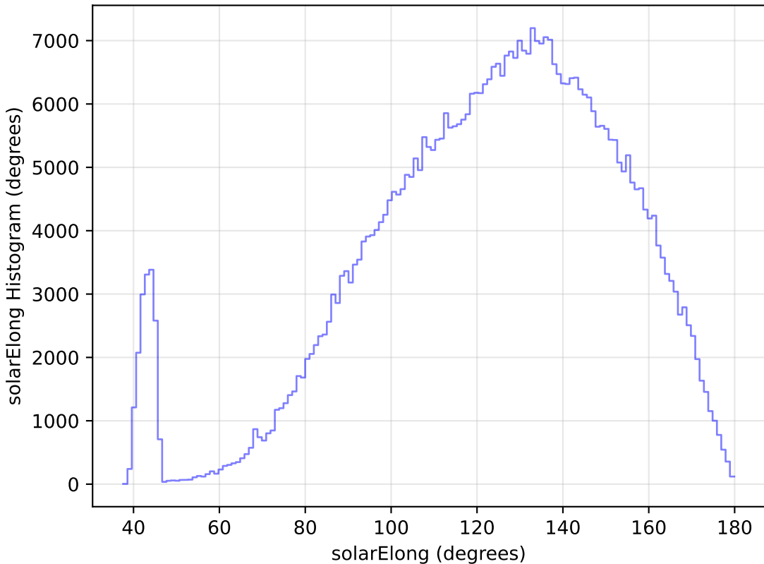
too_elab_r8_d3_giz_v3.4_10yrs All sky r band: solarElong Histogram
