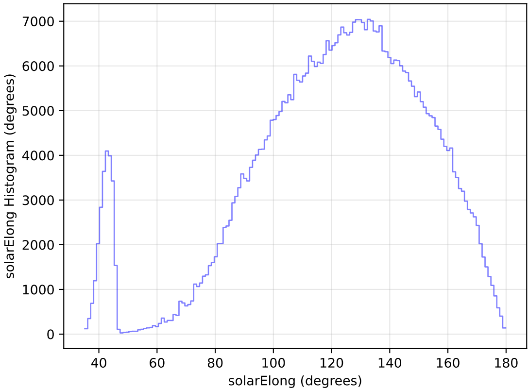
too_elab_r8_d3_giz_v3.4_10yrs All sky i band: solarElong Histogram
