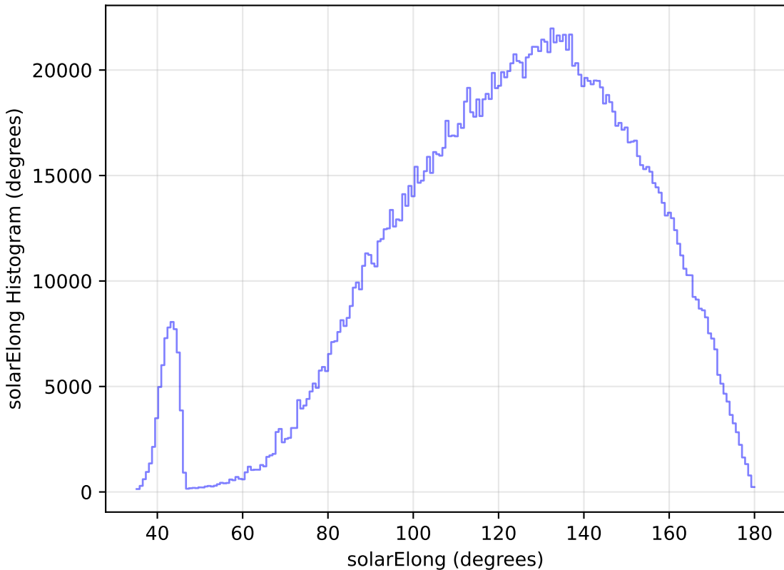
too_elab_r8_d3_giz_v3.4_10yrs All sky all bands: solarElong Histogram
