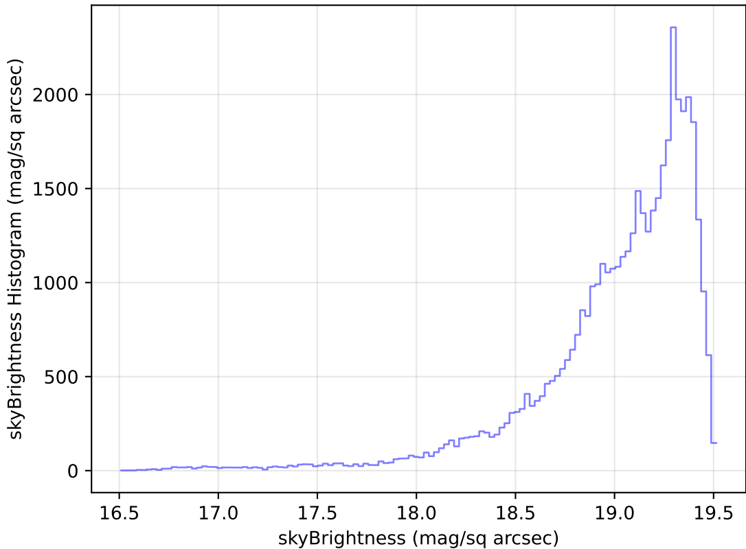
too_elab_r8_d3_giz_v3.4_10yrs Yr 1 z band: skyBrightness Histogram
