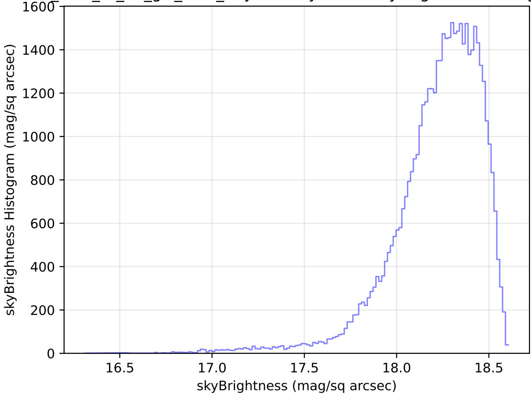
too_elab_r8_d3_giz_v3.4_10yrs Yr 1 y band: skyBrightness Histogram
