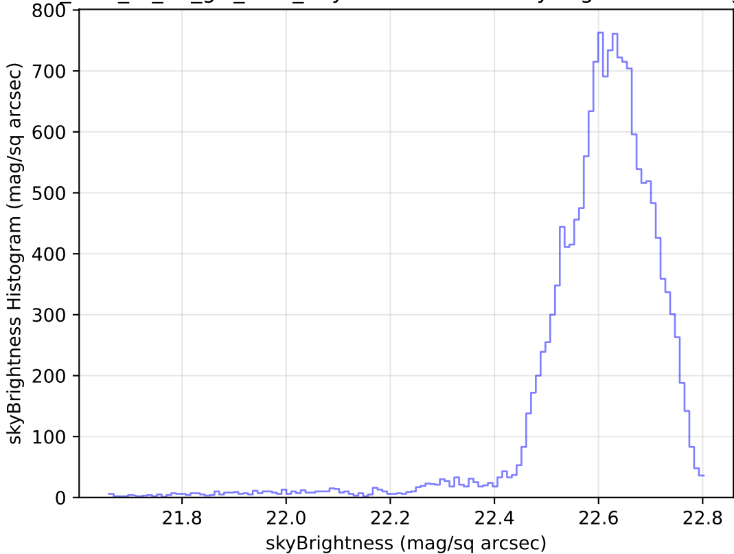
too_elab_r8_d3_giz_v3.4_10yrs Yr 1 u band: skyBrightness Histogram
