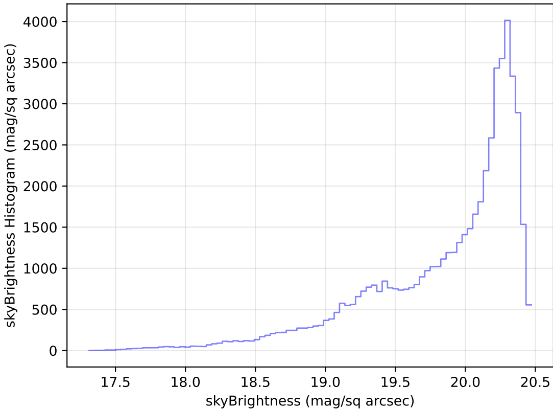
too_elab_r8_d3_giz_v3.4_10yrs Yr 1 i band: skyBrightness Histogram
