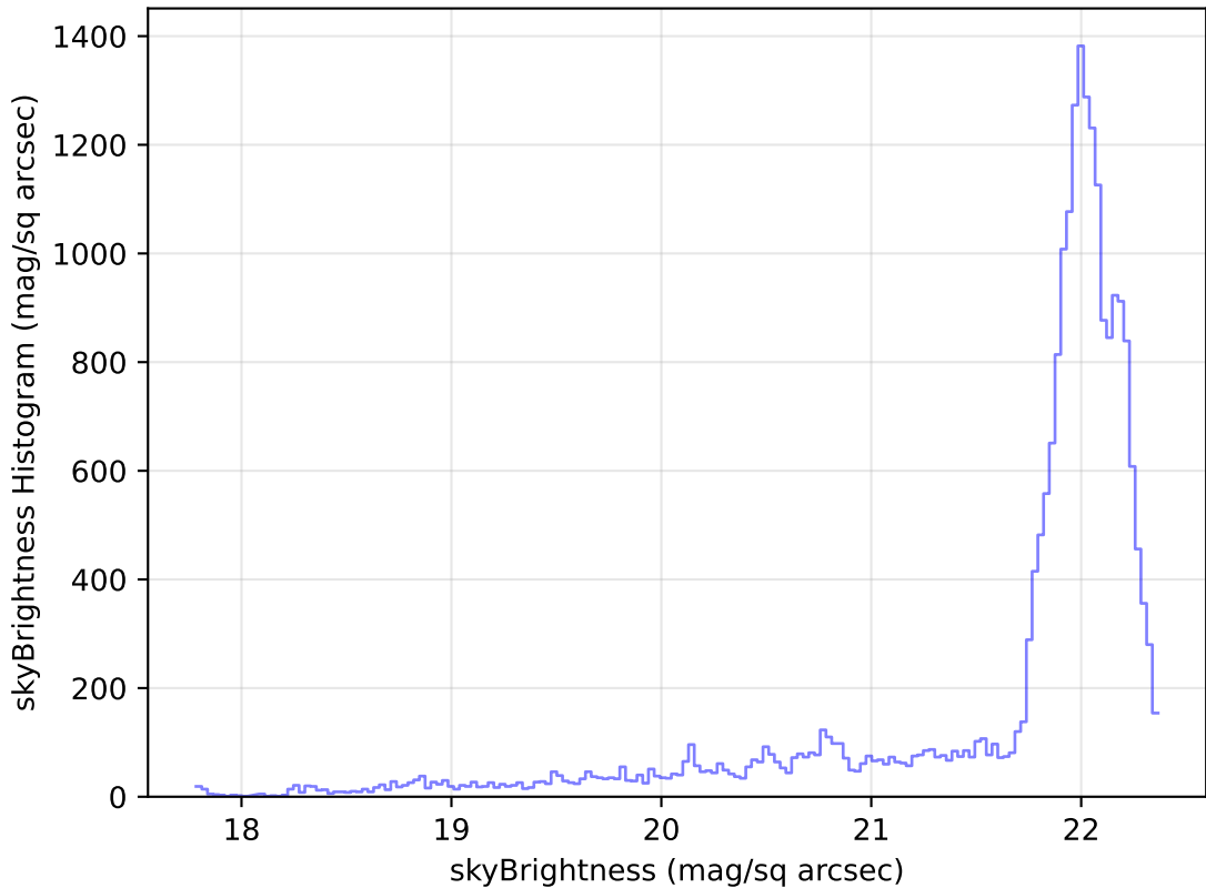
too_elab_r8_d3_giz_v3.4_10yrs Yr 1 g band: skyBrightness Histogram
