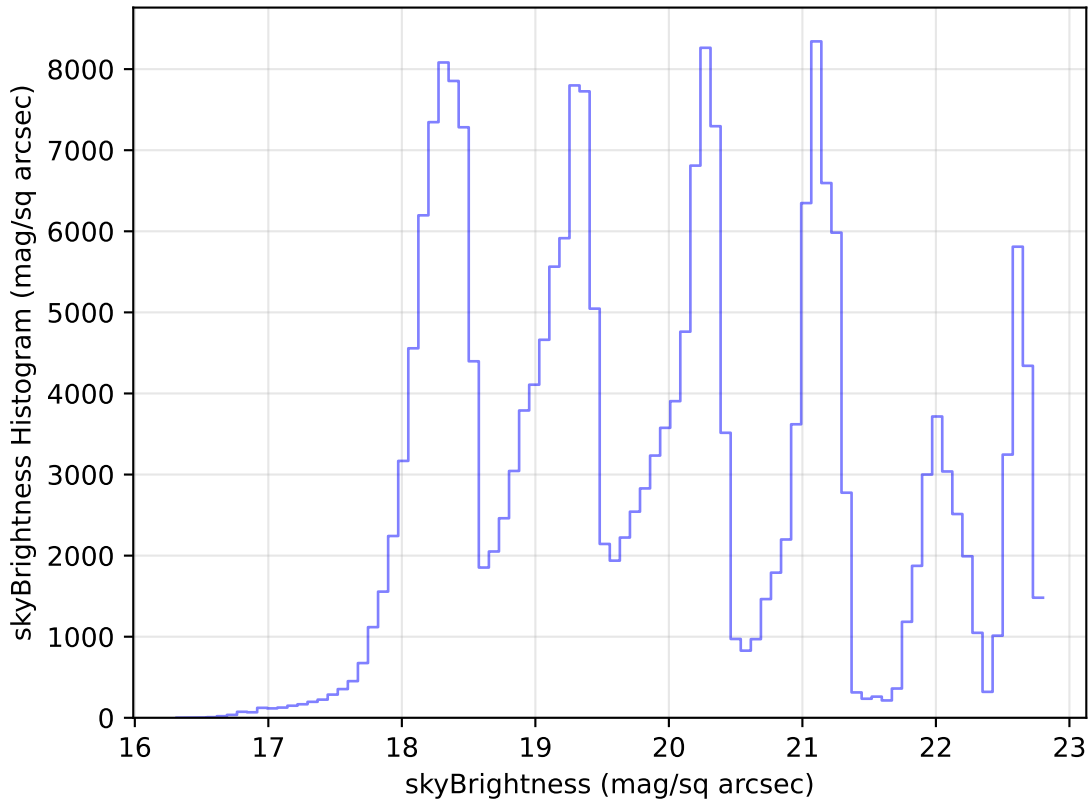
too_elab_r8_d3_giz_v3.4_10yrs Yr 1 all bands: skyBrightness Histogram
