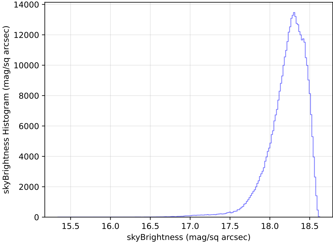
too_elab_r8_d3_giz_v3.4_10yrs WFD y band: skyBrightness Histogram
