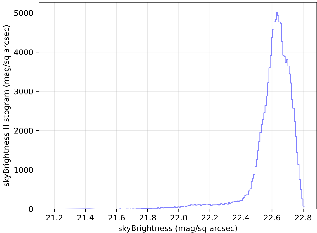
too_elab_r8_d3_giz_v3.4_10yrs WFD u band: skyBrightness Histogram
