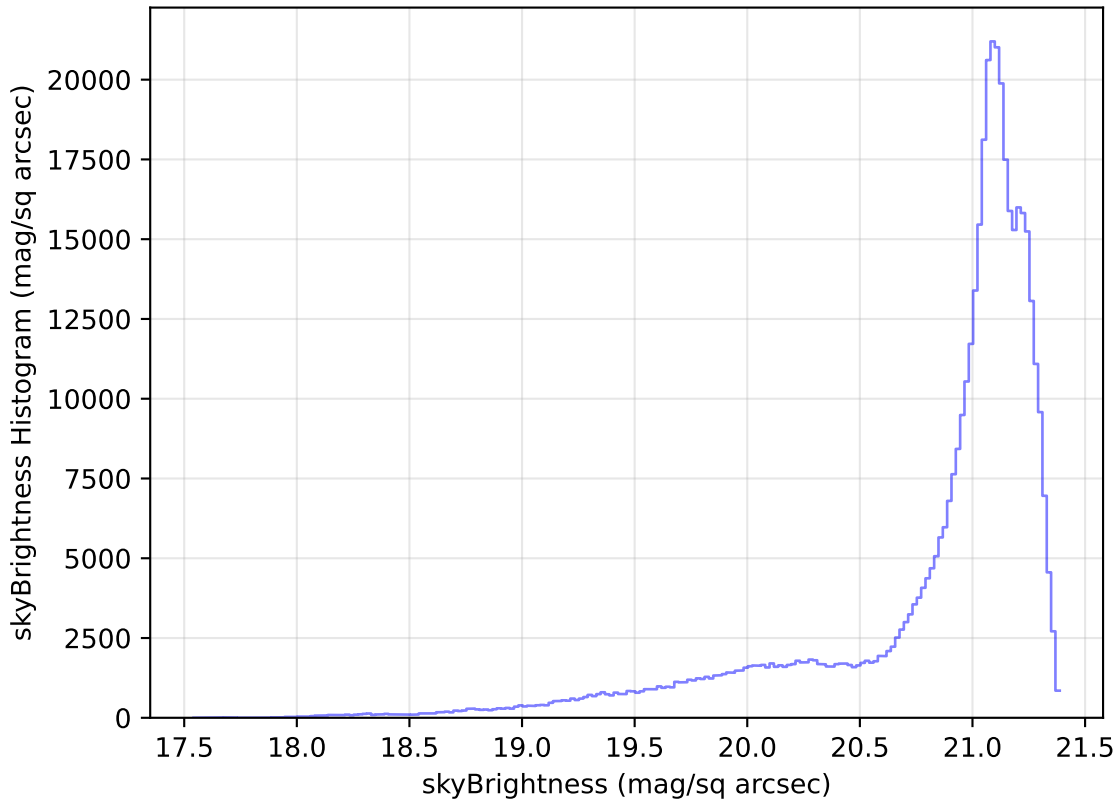
too_elab_r8_d3_giz_v3.4_10yrs WFD r band: skyBrightness Histogram
