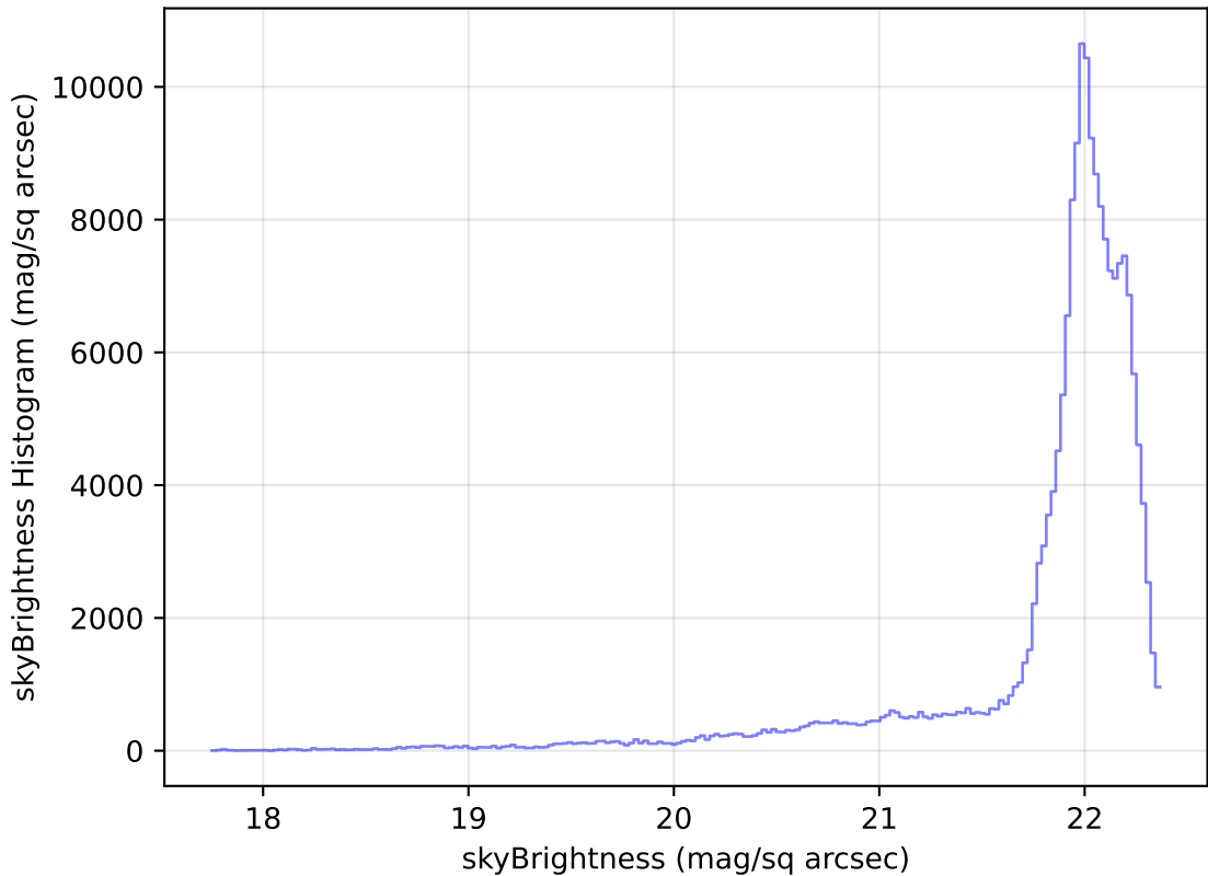
too_elab_r8_d3_giz_v3.4_10yrs WFD g band: skyBrightness Histogram
