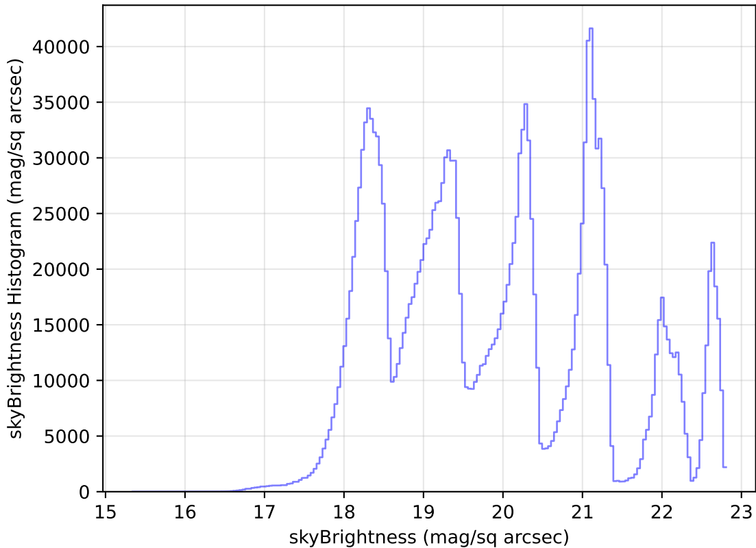
too_elab_r8_d3_giz_v3.4_10yrs WFD all bands: skyBrightness Histogram
