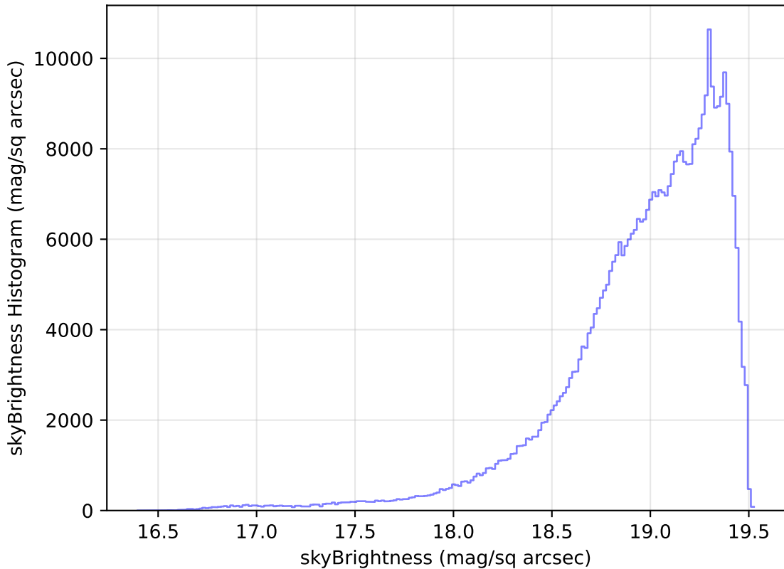
too_elab_r8_d3_giz_v3.4_10yrs All sky z band: skyBrightness Histogram
