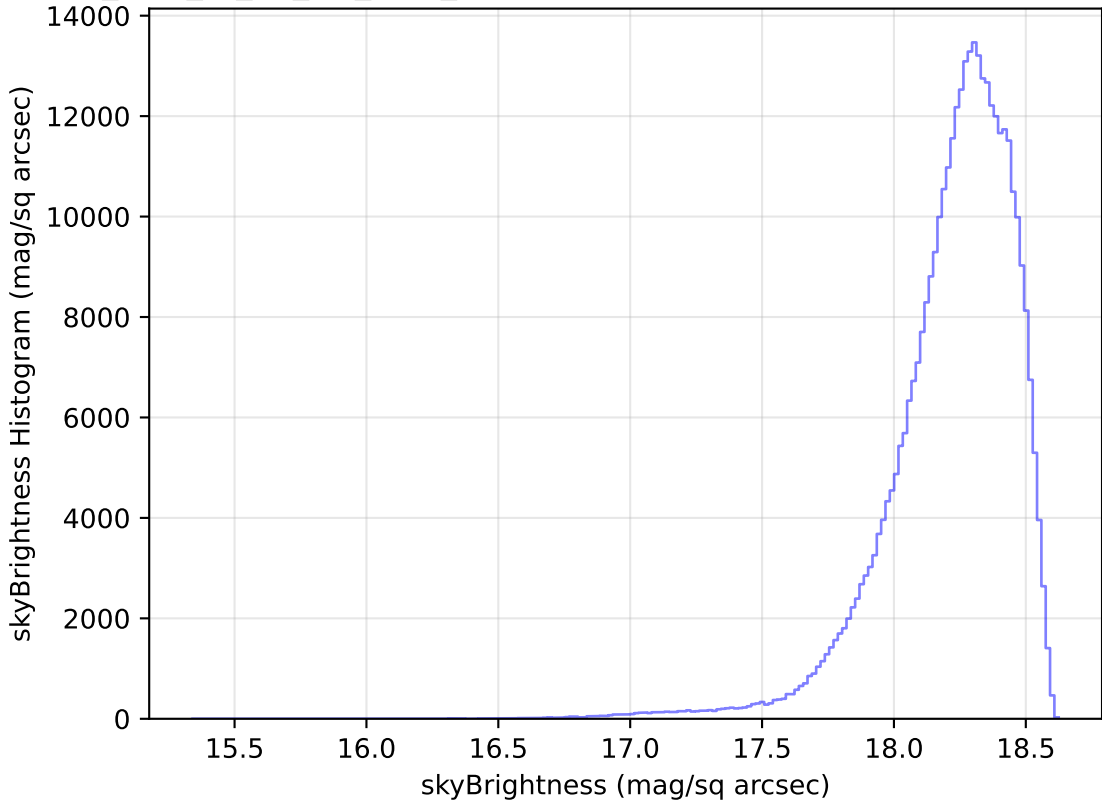
too_elab_r8_d3_giz_v3.4_10yrs All sky y band: skyBrightness Histogram
