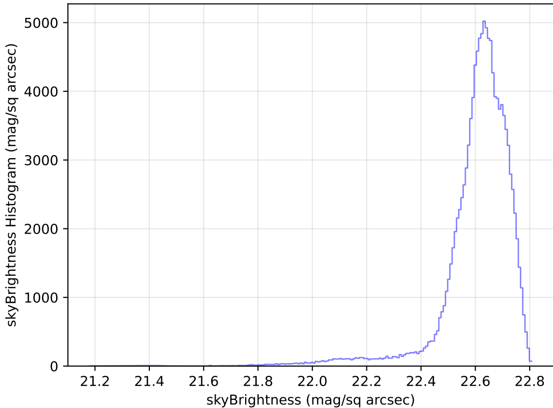
too_elab_r8_d3_giz_v3.4_10yrs All sky u band: skyBrightness Histogram
